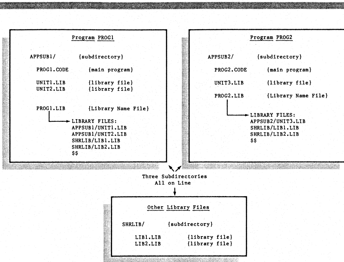
Figure 2-2. Designating Shared Libraries
